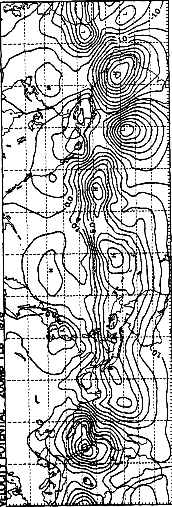
VELOCITY POTENTIAL 200MB FEB 1979
